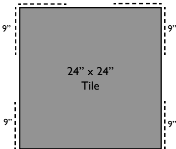
Tile to Tile CX-948 Placement 1/4" wide bead 9" in from all 4 edges.
